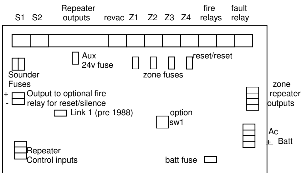
TYPICAL WIRING DETAILS
